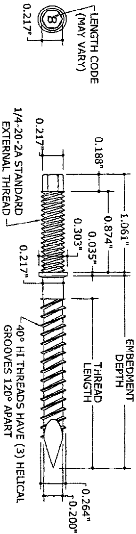
1 "TAPCON SG" SCREW 1:1 SCALE TOP & SIDE VIEWS
